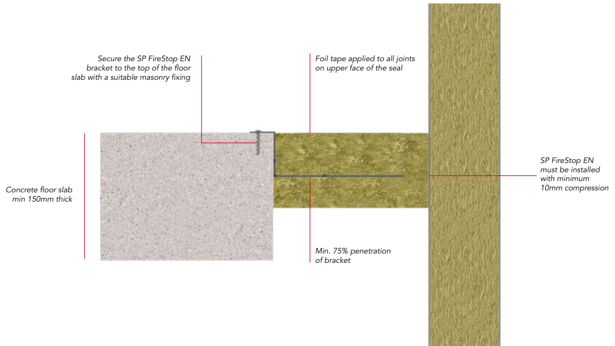
SP FireStop EN fixed to concrete floor slab
